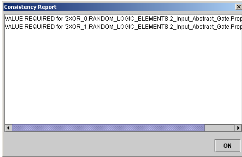
Figure 55. Consistency Report
