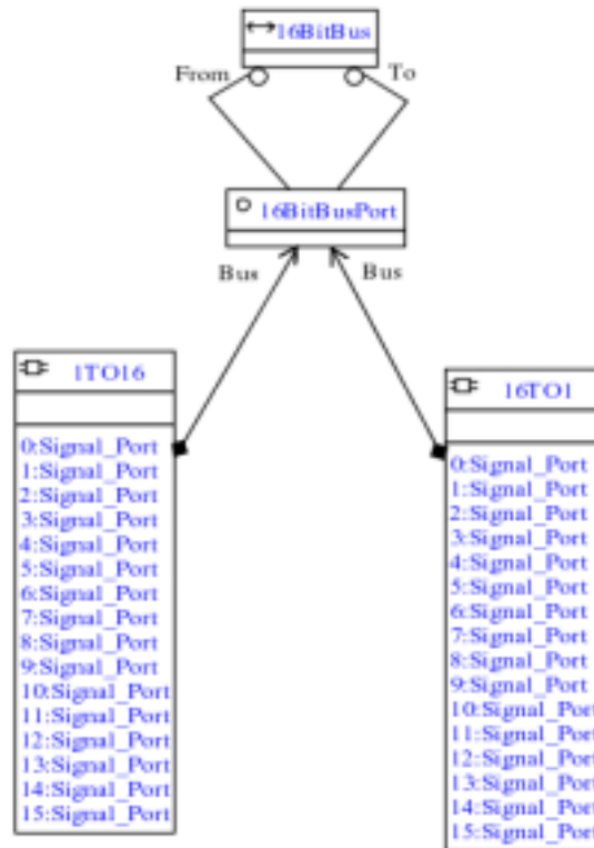
Figure 57. Bus Structures
